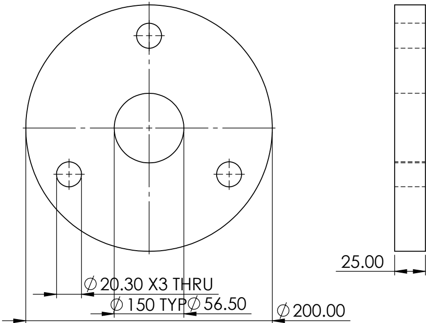
Retainer
