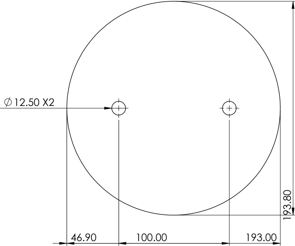
Plate
